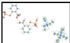
Fig. 1. Thermal ellipsoid plot (Barbour, 2001) of 3[(C_2H_5)_4N]^+ [H(C_6H_4O_5S_2)_2]^{3-} at the 50% probability level; hydrogen atoms are drawn as spheres of arbitrary radius. The dashed line denotes a hydrogen bond.
